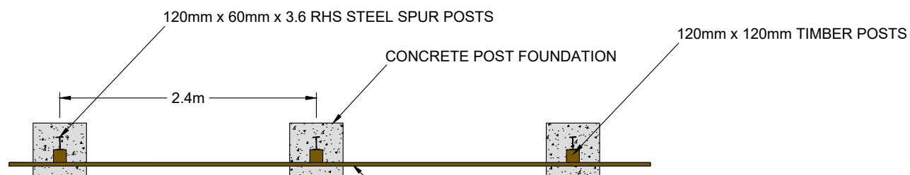
PLAN
