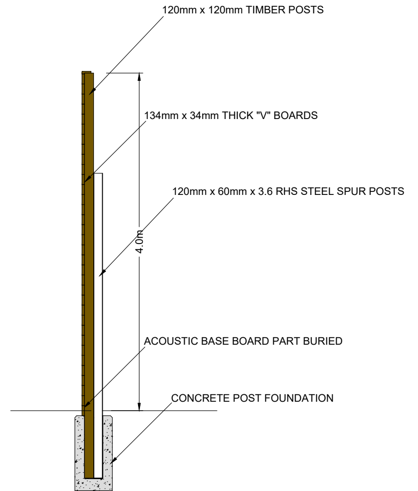
SECTION
