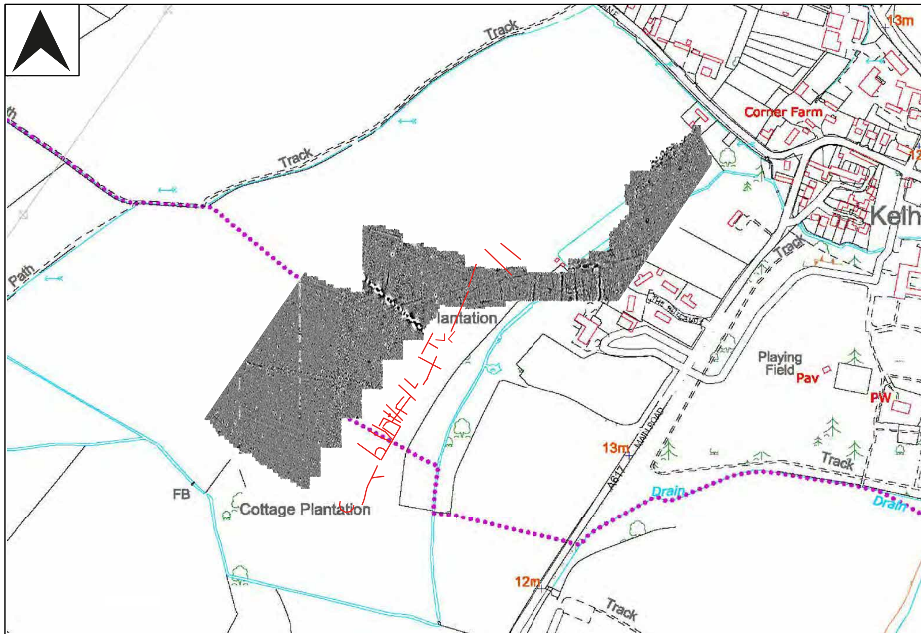
Figure 11. Field B +-3nT
