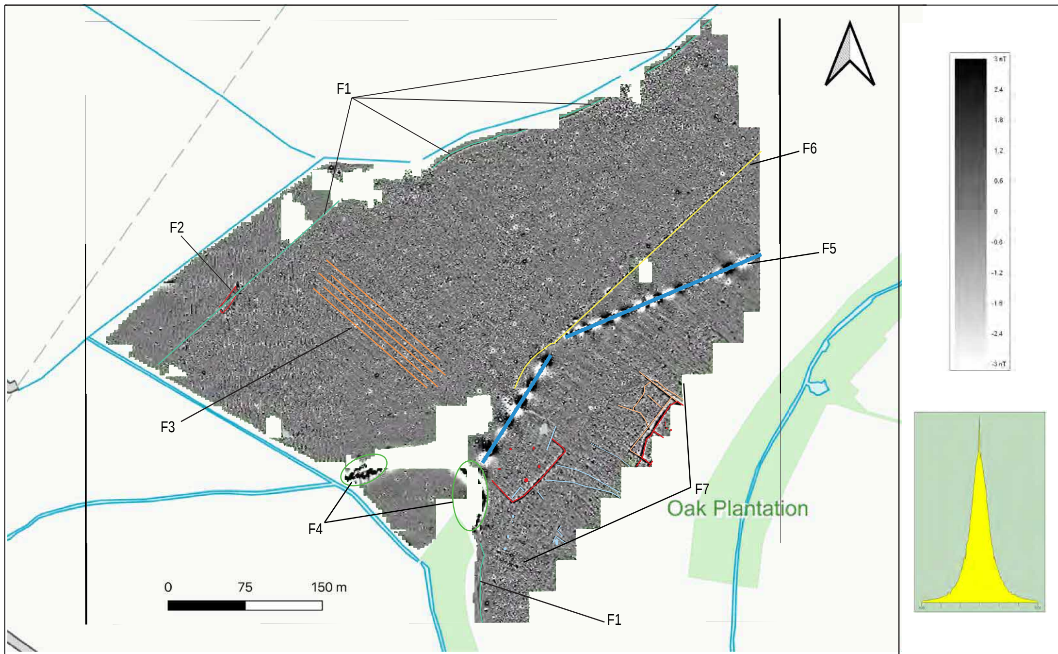
Figure 4. Survey Results annotated
