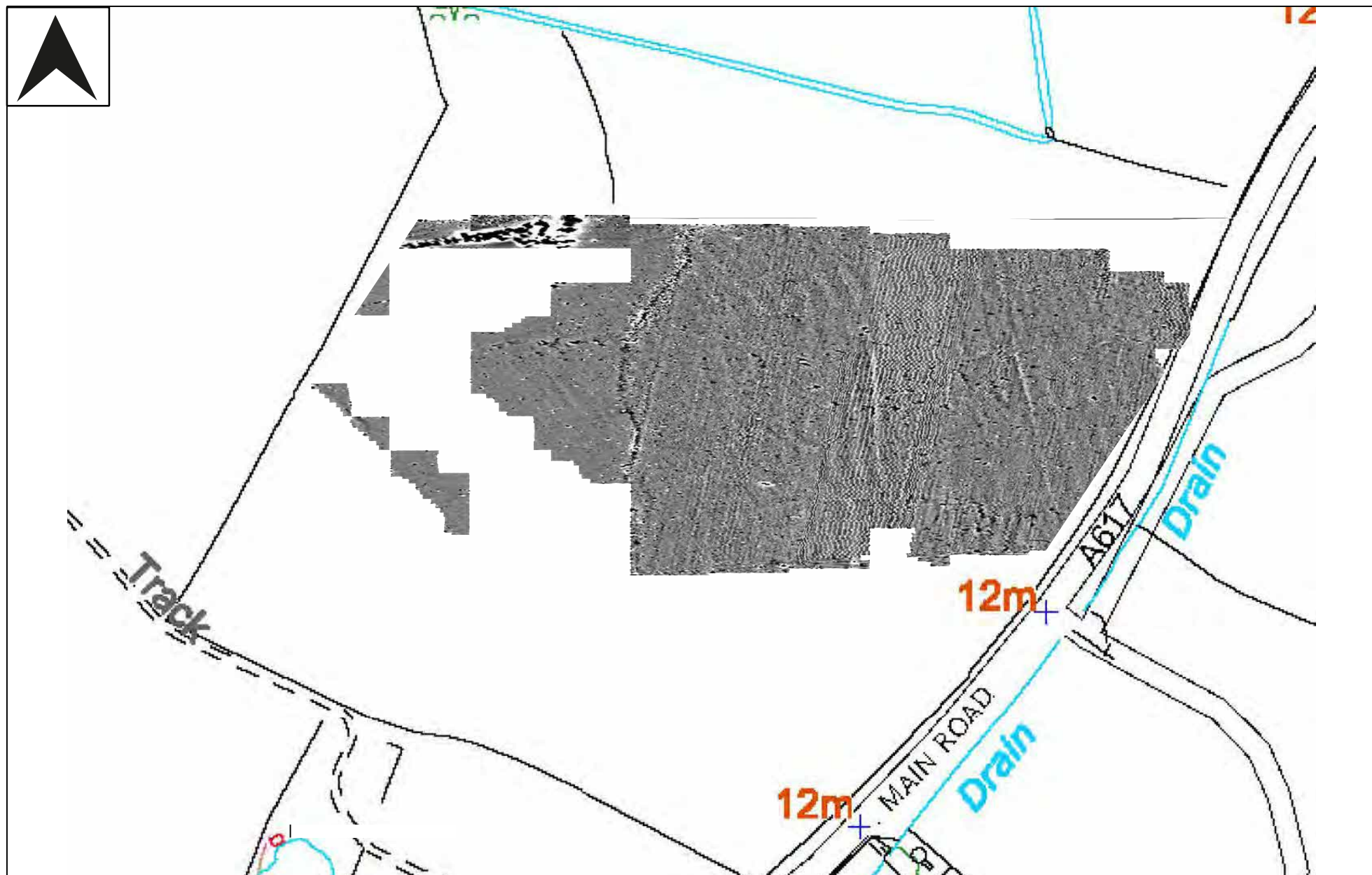
Figure 16. Field D +3nT
