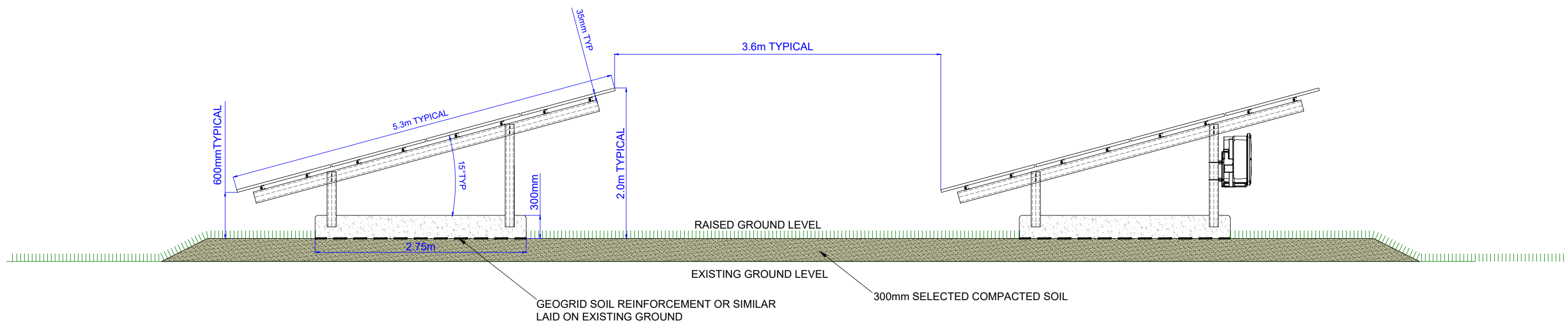
TYPICAL SECTION SLEEPER OPTION - ARCHAEOLOGY AREAS
