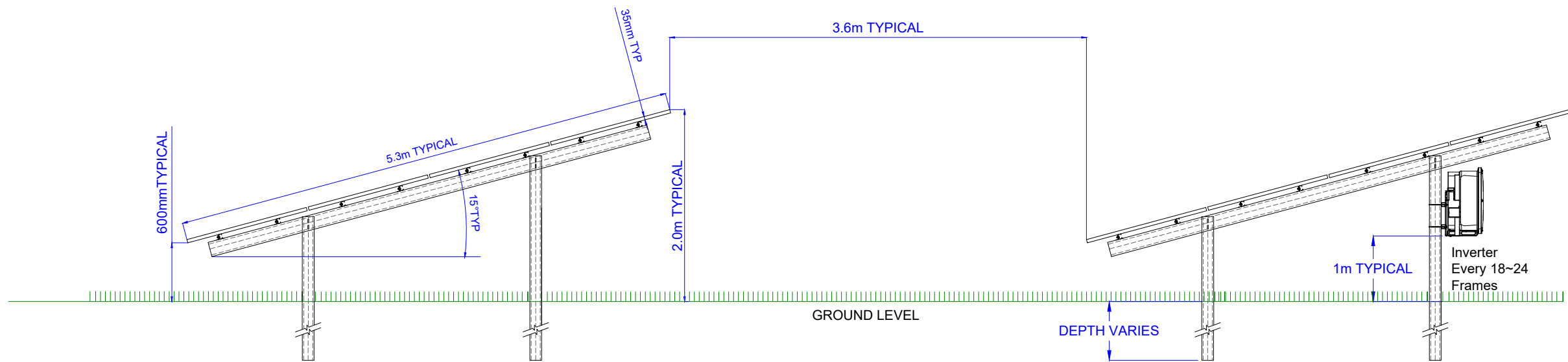
TYPICAL SECTION PILED OPTION
