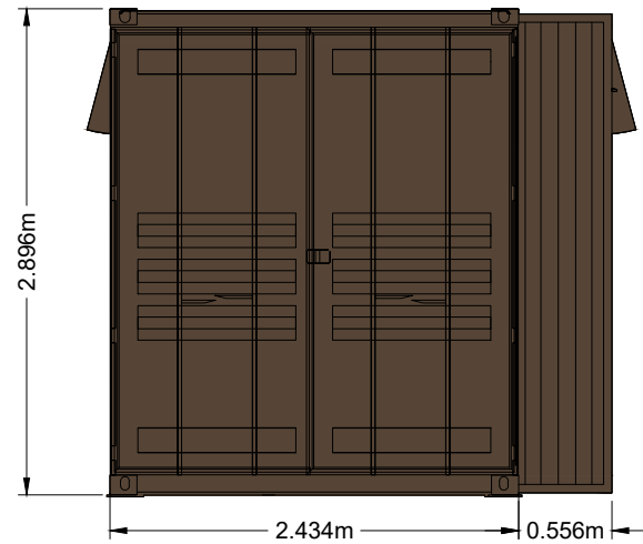
SOUTHERN ELEVATION
