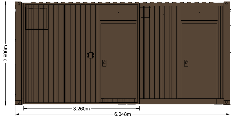
WESTERN ELEVATION
