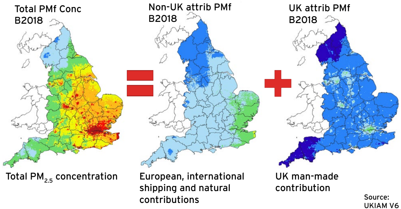
Figure 1. Maps of modelling outputs for 2018 produced by Imperial College London using the UK Integrated Assessment model showing how (a) variations in PM 2.5 from natural sources and sources from outside the UK and (b) UK manmade PM 2.5 result in significantly different concentrations across the country.
